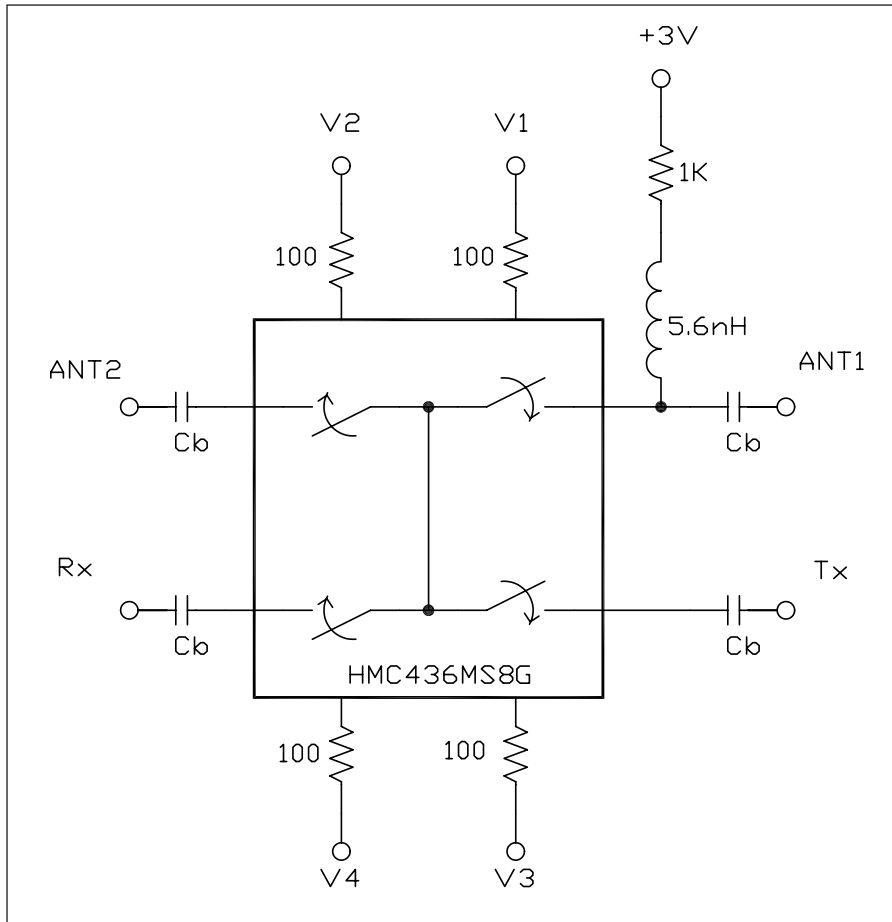
Figure 2 - Application Circuit
